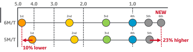
New 6-speed MANUAL transmission gear ratios
