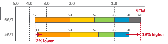
New 6-speed AUTOMATIC transmission gear ratios
