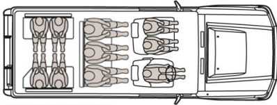
10 seats configuration
