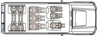
10 seats configuration
