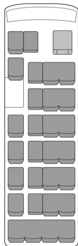
30 seats configuration
